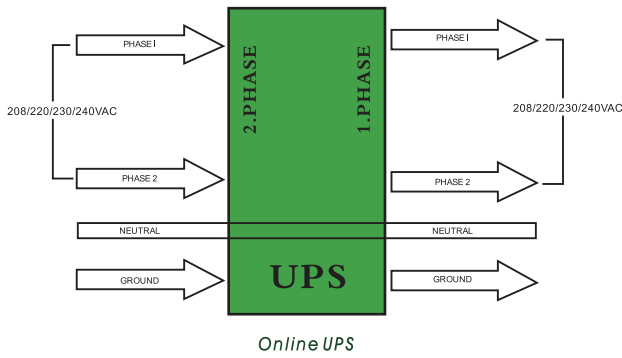
Online UPS
