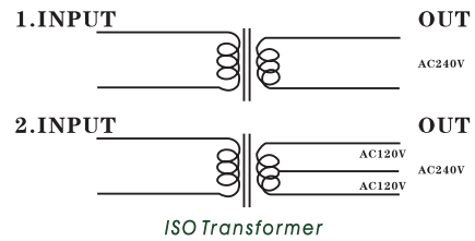
ISO Transformer
