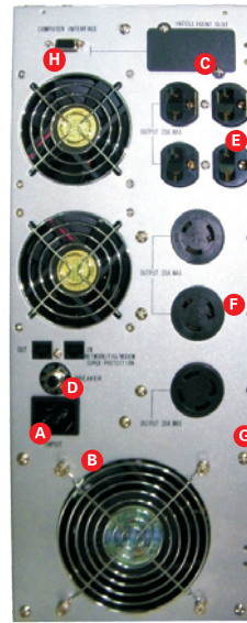
HP9116BC UPS
